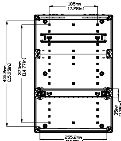
INTERIOR VIEW WITHOUT LID
