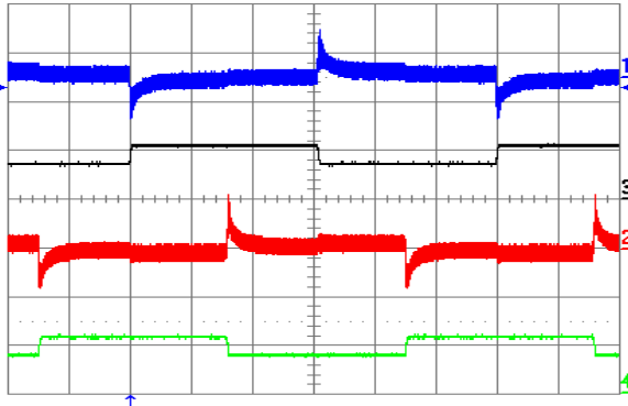
Figure 23. Output voltage response to both lout1 and lout2 (out of phase) load current step-change of 3.75 A (50%-75%-50%) at V_{in} = 48\text{ V} . Ch1 = Vout1 (50 mV/div), Ch2 = Vout2 (50 mV/div), Ch3 = lout1 (10 A/div.), Ch4 = lout2 (10 A/div.). Current slew rate: 0.1 A/ \mu\text{s} , C_o = 10\text{ }\mu\text{F} tantalum + 1 \mu\text{F} ceramic. Time scale: 1 ms/div.
