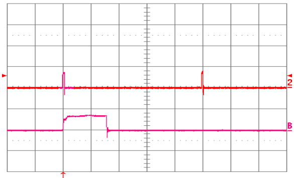
Figure 28. Load current lout2 into a 10 m \Omega short circuit on Vout2 during restart, with Vout1 open (no load), at V_{in} = 48\text{ V} . Ch2 = lout2 (20 A/div, 20 ms/div). ChB = lout2 (20 A/div, 1 ms/div) is an expansion of the on-time portion of lout2.
