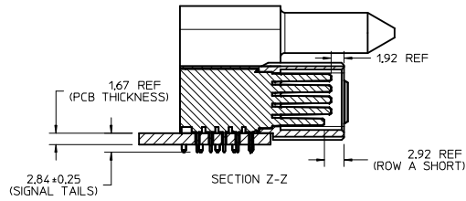
MATED PROFILE (MATED WITH VERT RECEPTACLE ASSY)
