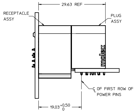
MATED PROFILE (MATED WITH VERT RECEPTACLE ASSY)
