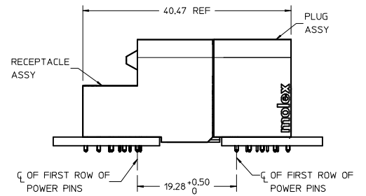
MATED PROFILE (MATED WITH R/A RECEPTACLE ASSY)
