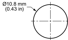
Figure 2. ANT-2.4-WRT-MON Series Antenna Recommended Enclosure Mounting Dimensions
