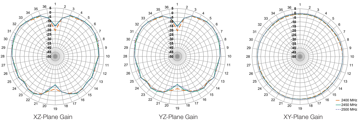
Figure 9. ANT-2.4-WRT-MON Radiation Patterns
