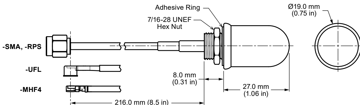
Figure 1. ANT-2.4-WRT-MON Antenna Dimensions
