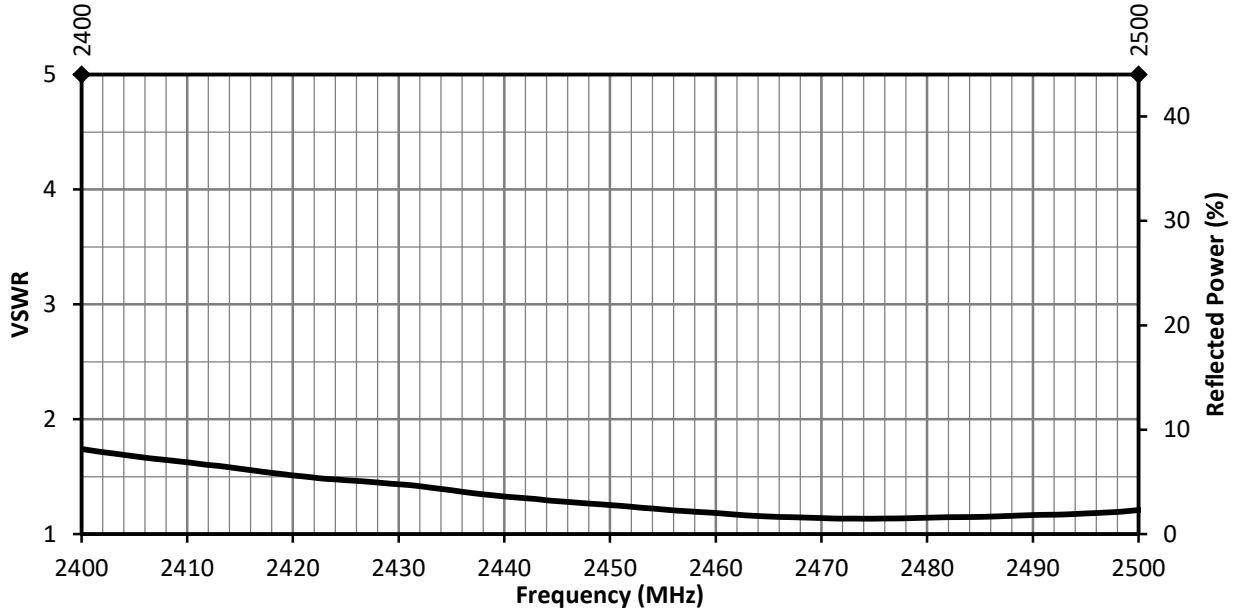
Figure 4. ANT-2.4-WRT-MON VSWR
