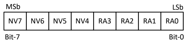
Figure 7-6. Resistor Address
