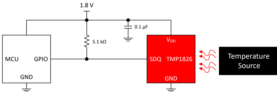
Figure 8-2. Supply Powered Application
