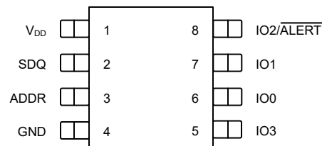
Figure 5-2. DGK 8-Pin VSSOP Top View
