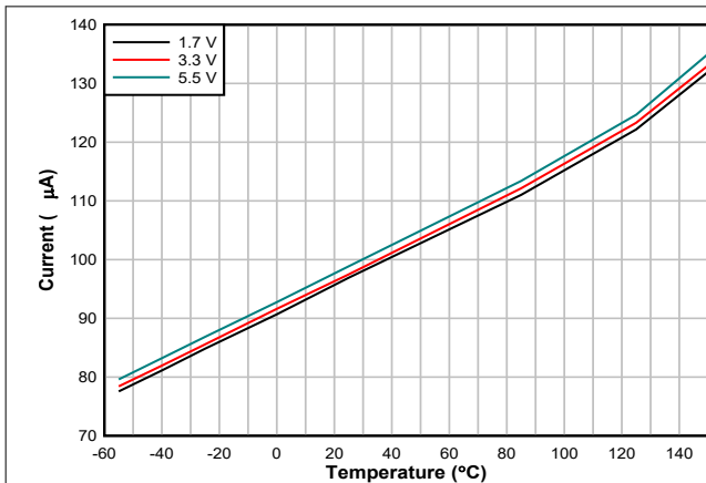
Figure 6-9. Temperature Conversion Current vs Temperature
