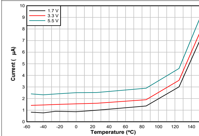
Figure 6-9. Temperature Conversion Current vs Temperature
