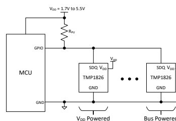
Simplified Schematic
