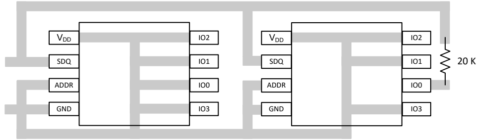
Figure 8-5. IO Hardware Address in Bus Powered Mode
