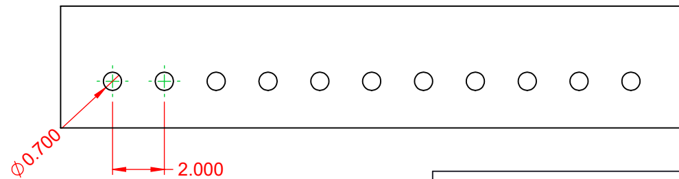
SUGGESTED PCB LAYOUT
