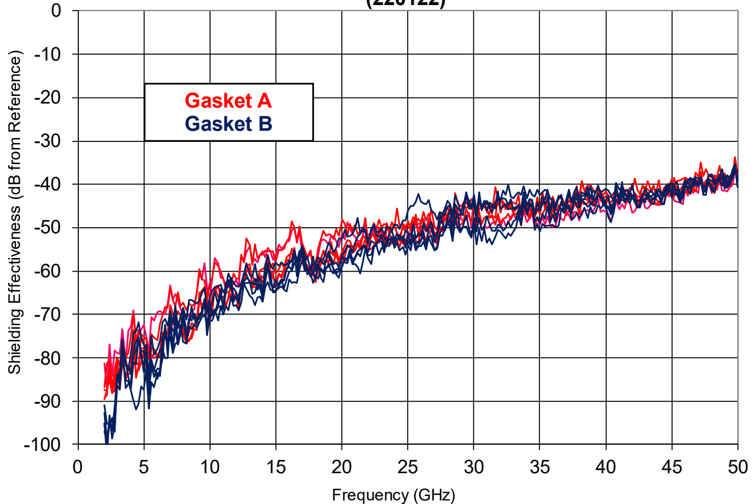
zSFP+ 2x4 Gasket Test Fixture, Gasket A vs Gasket B (220122)
