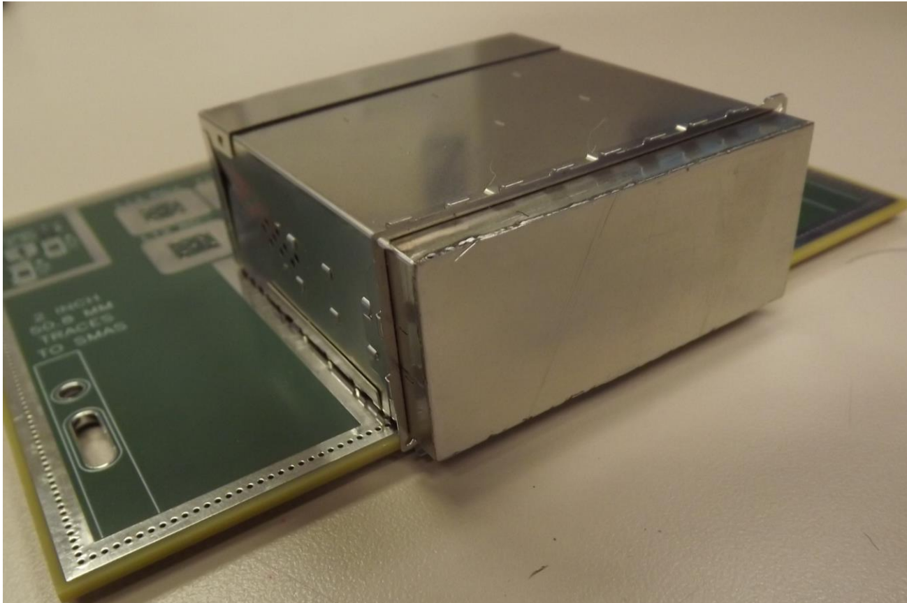
Sealed zSFP+ 2x4 Cage Test Fixture
