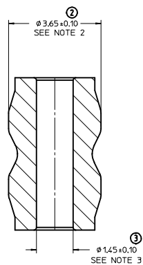
SECTION Y-Y SCALE 15:1
