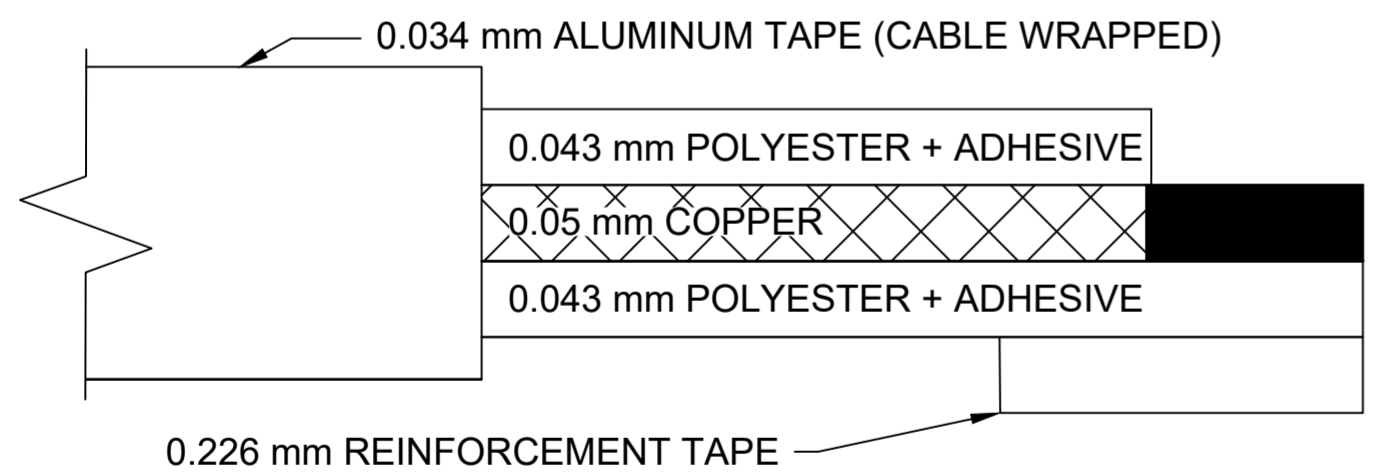
CROSS-SECTION
