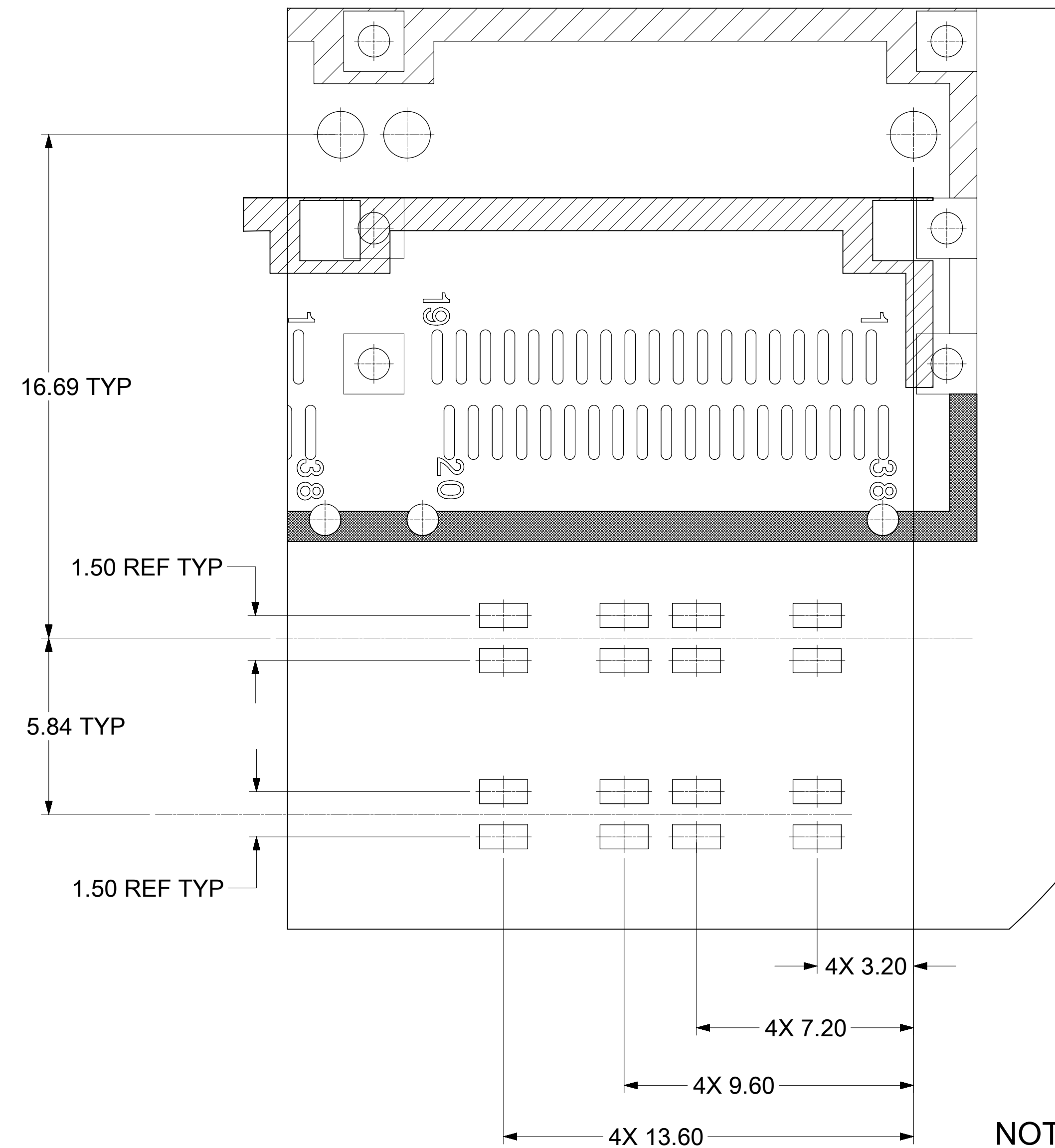
Detail 1 Scale 8:1
