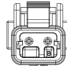
KEY-B CONFIGURATION ATMH06-2SB TPA COLOR: BLACK
