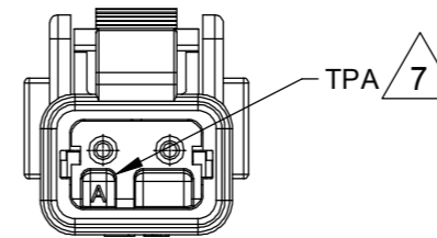
KEY-A CONFIGURATION ATMH06-2SA TPA COLOR: GRAY
