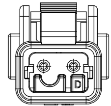
KEY-D CONFIGURATION ATMH06-2SD TPA COLOR: BROWN
