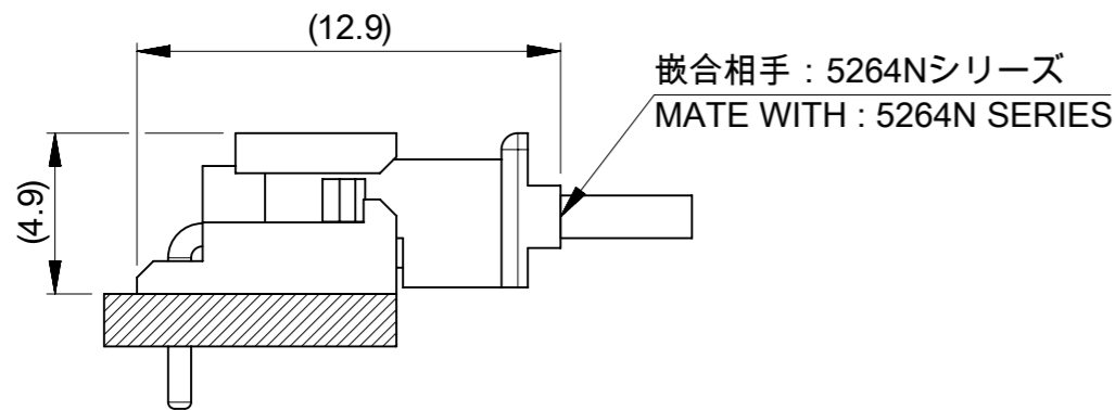
2-8極 2-8 CIRCUIT
