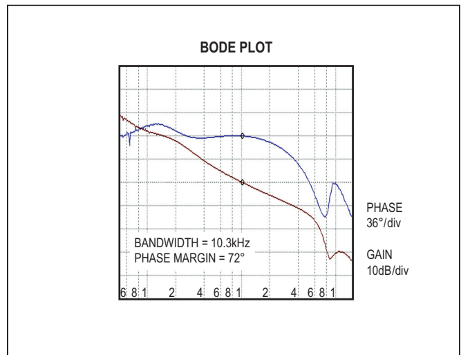
Figure 4. Bode Plot
