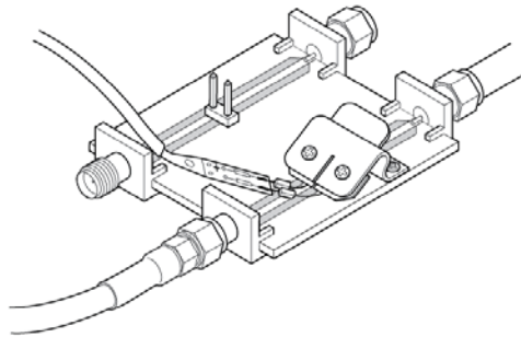
SI Lead connected to Deskew Fixture
