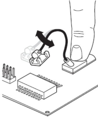
Applying pressure when adjusting the probe holder
