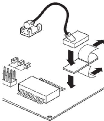
Connecting the SI Module Using the Tip Retaining Clip
