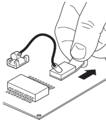
Removing the retaining clip
