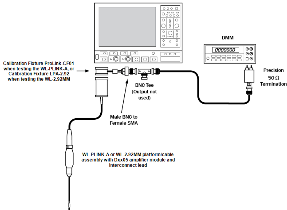
Output Zero test setup
