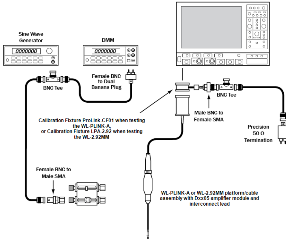
DC Frequency Attenuation Test Setup
