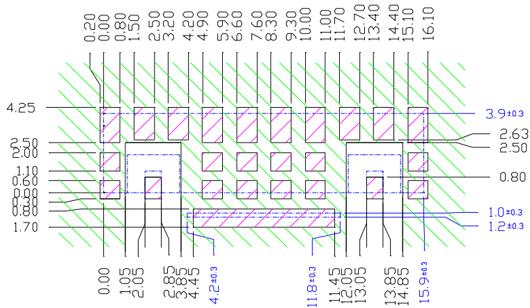
PCB Layout
