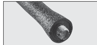
SMA F T2 SMA Female recessed Insulator & partial(long) skirt (SFU type)
