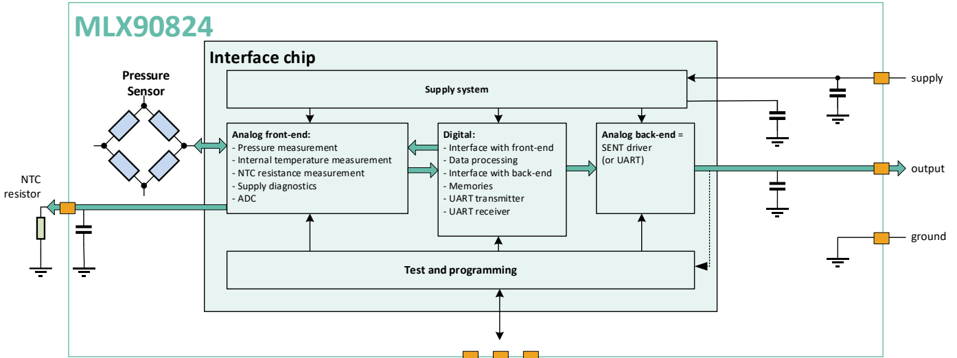
Figure 5: MLX90824 functional block diagram
