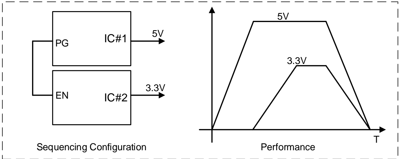
Figure 39. Sequencing Configuration
