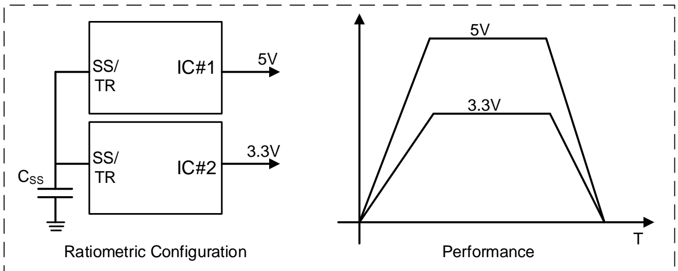
Figure 37. Ratiometric Configuration
