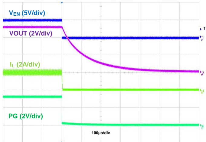
Figure 34. Shutdown using EN with PG, IOUT = 2A
