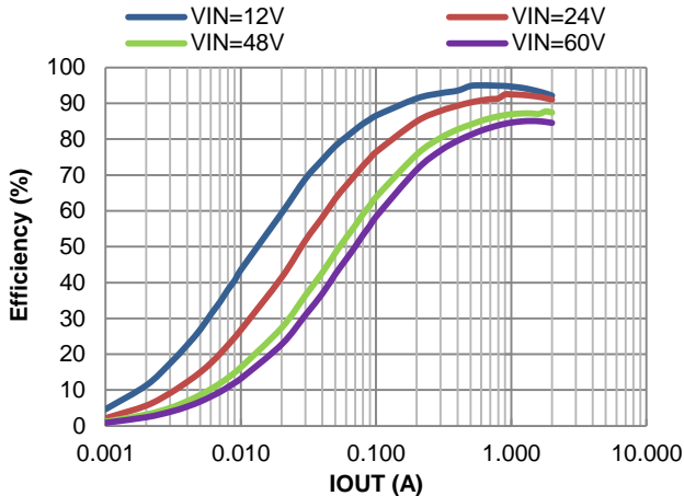
Figure 6. PWM Efficiency vs. Output Current, V_{OUT}=5\text{V} , L=10\mu\text{H}
