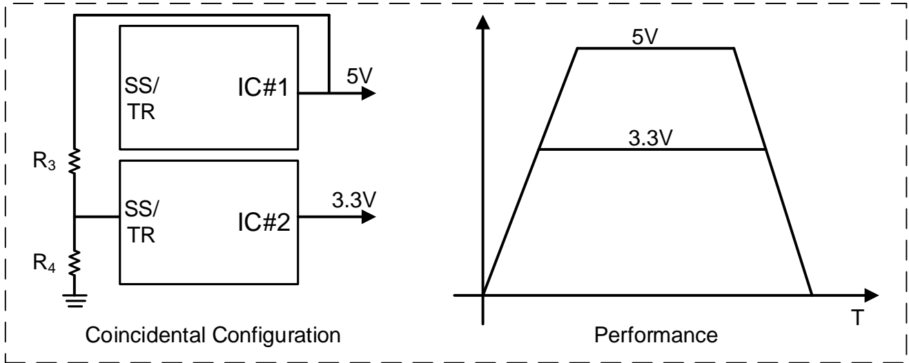
Figure 38. Coincidental Configuration
