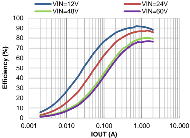
Figure 8. PWM Efficiency vs. Output Current, V_{OUT}=3.3\text{V} , L=8.2\mu\text{H}
