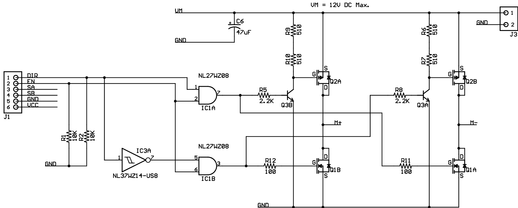
Motor Connections
