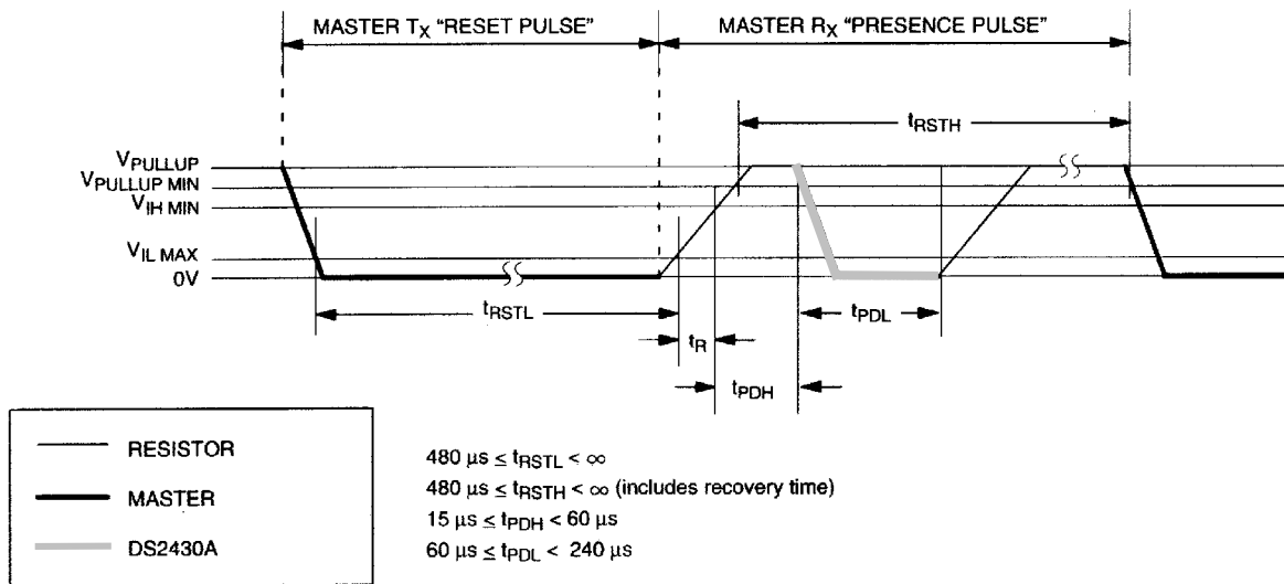
INITIALIZATION PROCEDURE "RESET AND PRESENCE PULSES" Figure 9
