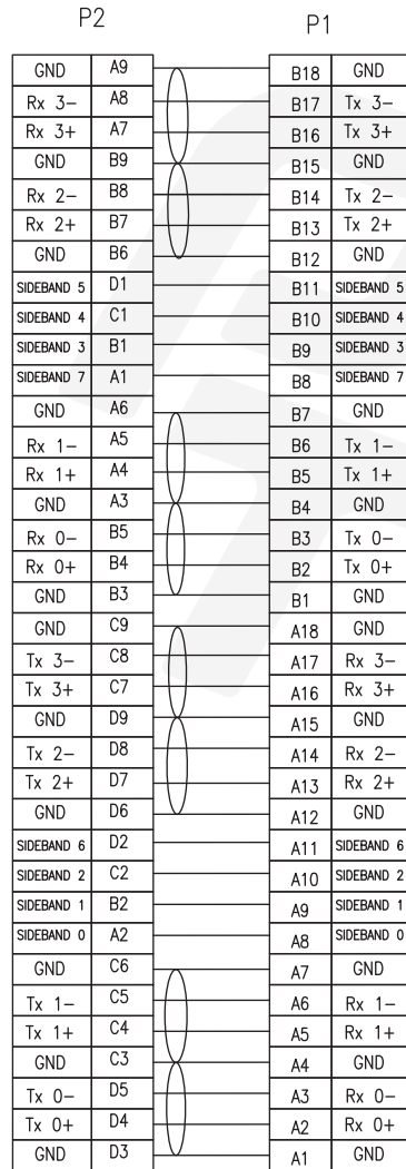
WIRING DIAGRAM
