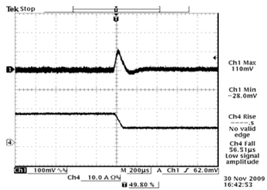
Figure 14. 50%-25% Load Transients at V_{in}=24V , V_{out}=5V
