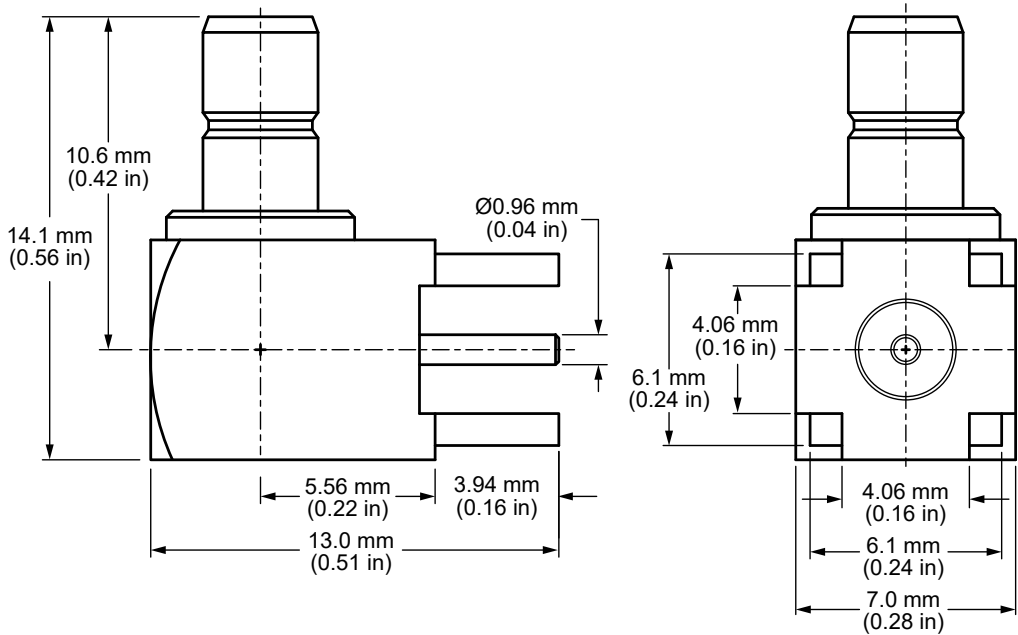
Figure 1. Product Dimensions for the CONSMB002-G Connector
