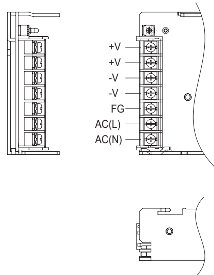
Fig.5.1 Example of option -T (PMA100F)
