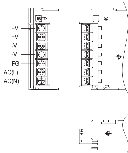
Fig.5.2 Example of option -T1 (PMA100F)
