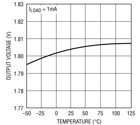
Output Voltage
