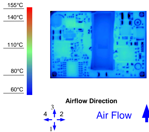
Figure 8. Thermal Image for Airflow Direction 3 (12A output, 55°C ambient, 200 LFM, typical Vin, open frame, unit soldered onto a fixture board)
