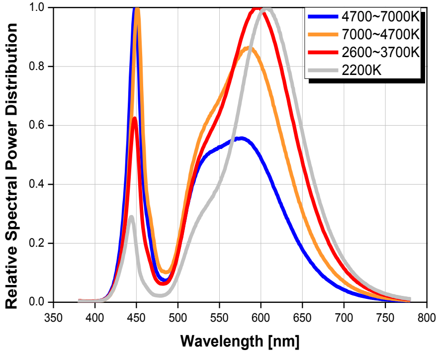
Fig 1. Color Spectrum, T_j=25^\circ\text{C} , I_F=640\text{mA} (CRI70)
