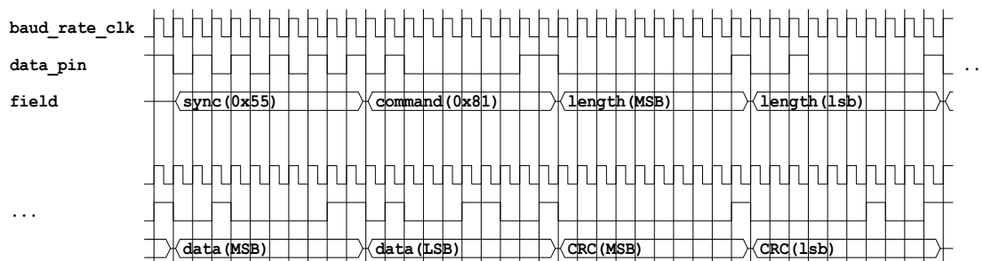
Figure 39-9. Example Command
