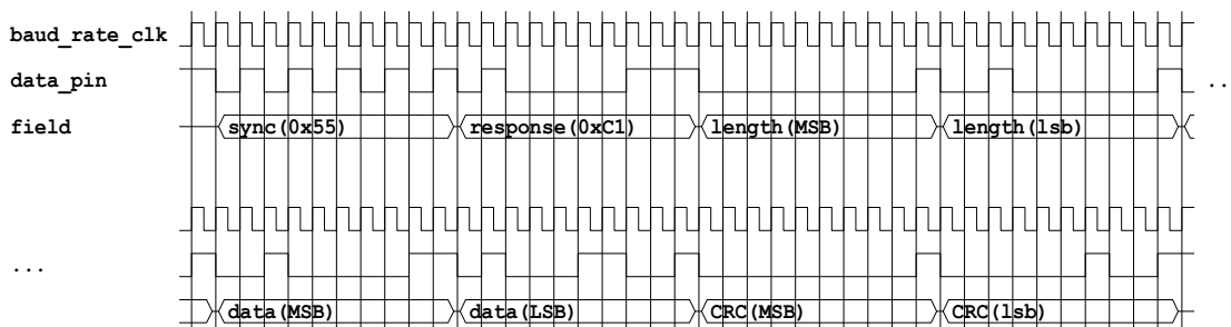
Figure 39-10. Example Response
