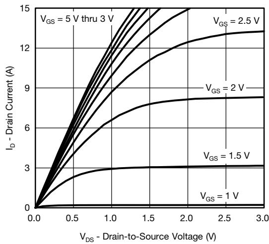
Output Characteristics
