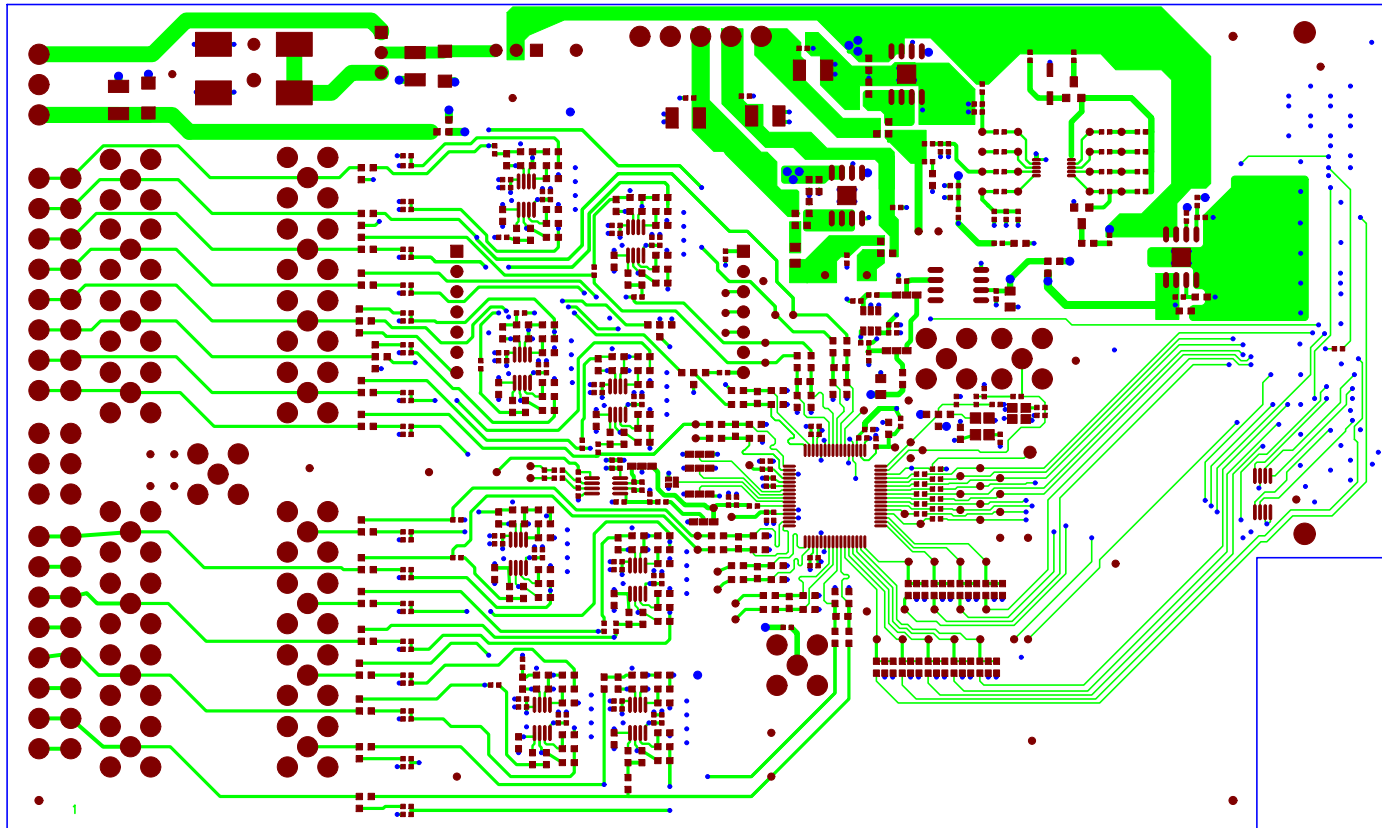
EVAL-AD7768FMCZ Rev. A - Component Side View Layer 1 - Component Side (Primary)
