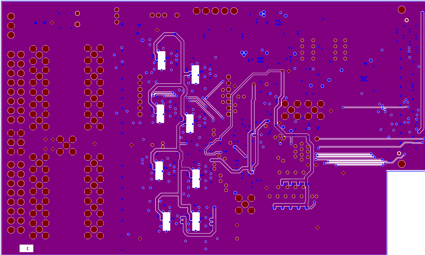
EVAL-AD7768FMCZ Rev. A – Component Side View
