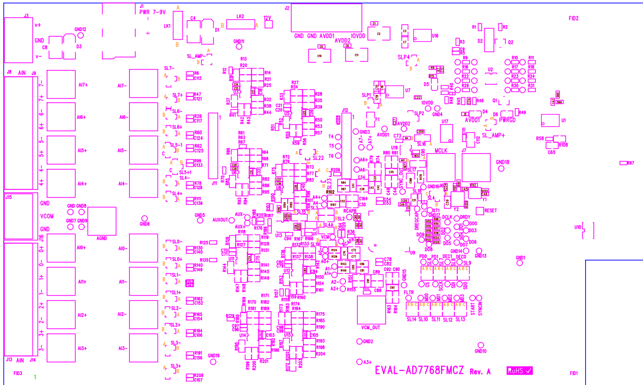
EVAL-AD7768FMCZ Rev. A – Component Side View Layer 1 – Component Side (Primary) Silkscreen Top
