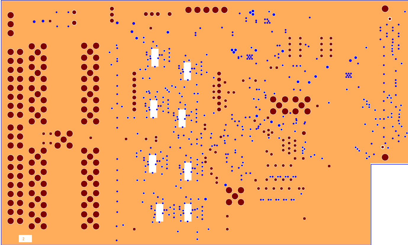
EVAL-AD7768FMCZ Rev. A - Component Side View Layer 2 - GND Planes
