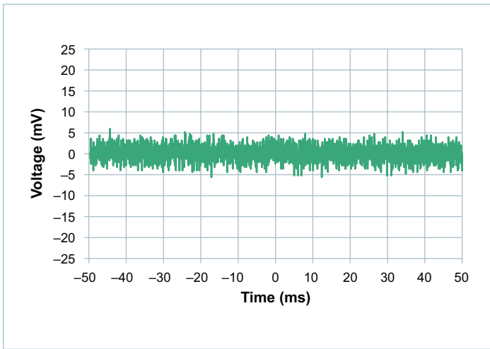
Figure 23 — AUX1 (-12V) ripple with no load, AC-coupled
