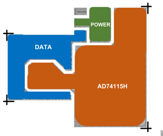
Figure 2. Isolation Zones on the EVAL-AD74115H-ARDZ
