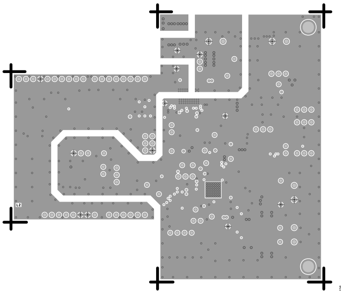
Figure 25. Layer 2, Ground Layer
