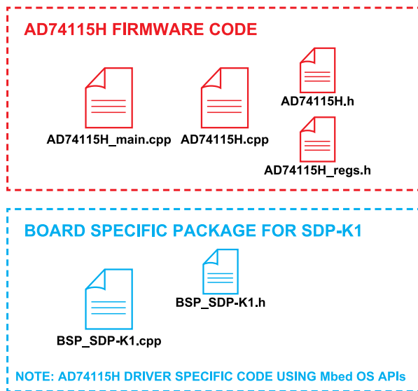
Figure 18. AD74115H No-OS Firmware Structure
