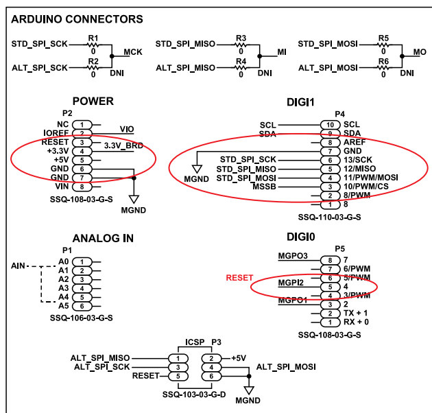
Figure 19. Arduino Connector During User-Defined SPI Setup
