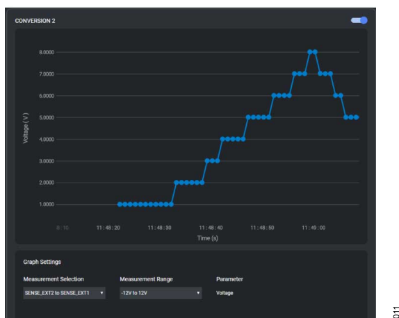
Figure 11. Differential Voltage Measurement Example
