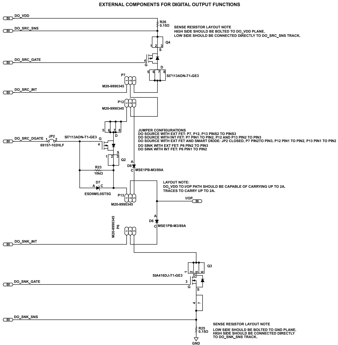
Figure 23. Digital Output Circuitry
