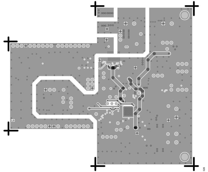
Figure 26. Layer 3, Power Layer
