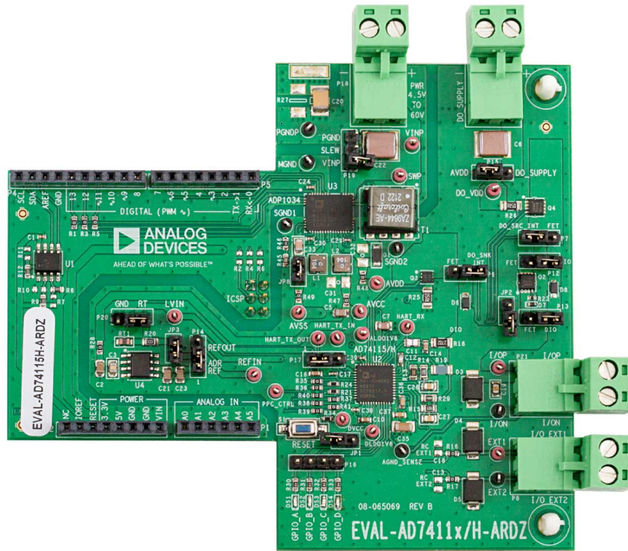
Figure 1. Evaluation Board Photograph
