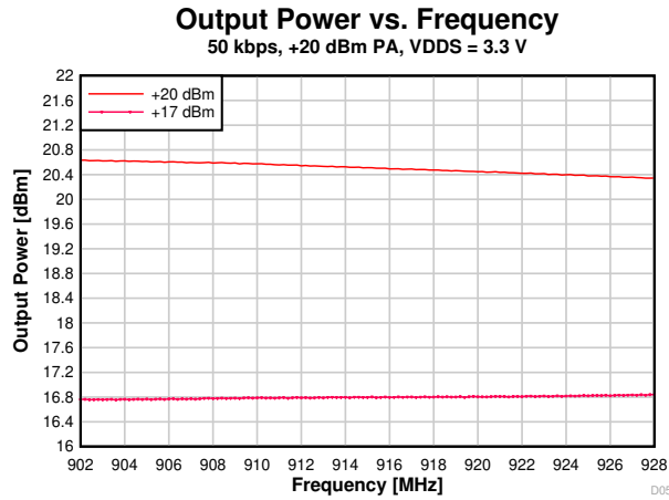
Figure 8-27. Output Power vs. Frequency (50 kbps, 915 MHz, VDD5 = 3.3 V)
