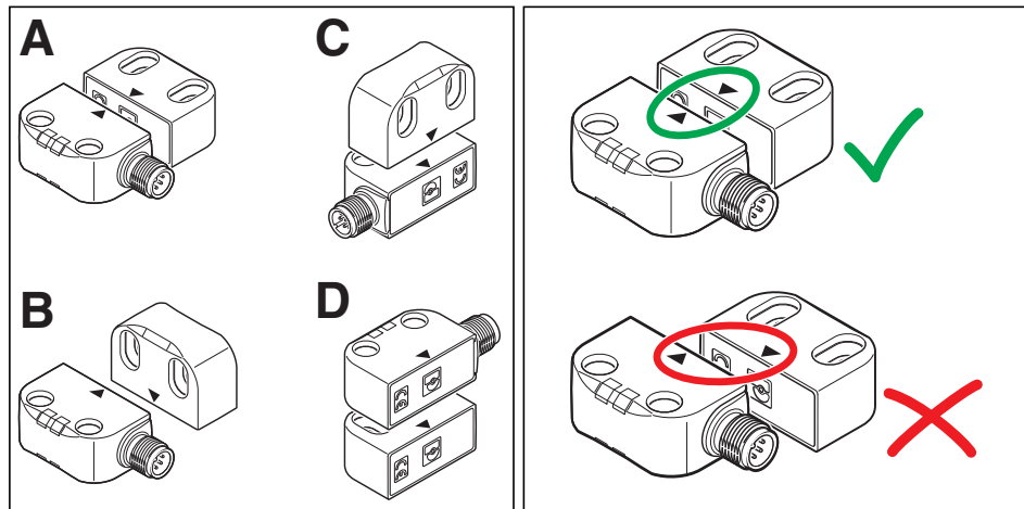
Figure 2-4 Actuation positions
