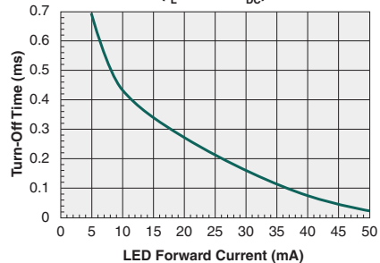
Typical Turn-Off Time vs. LED Forward Current (I L =120mA DC )
