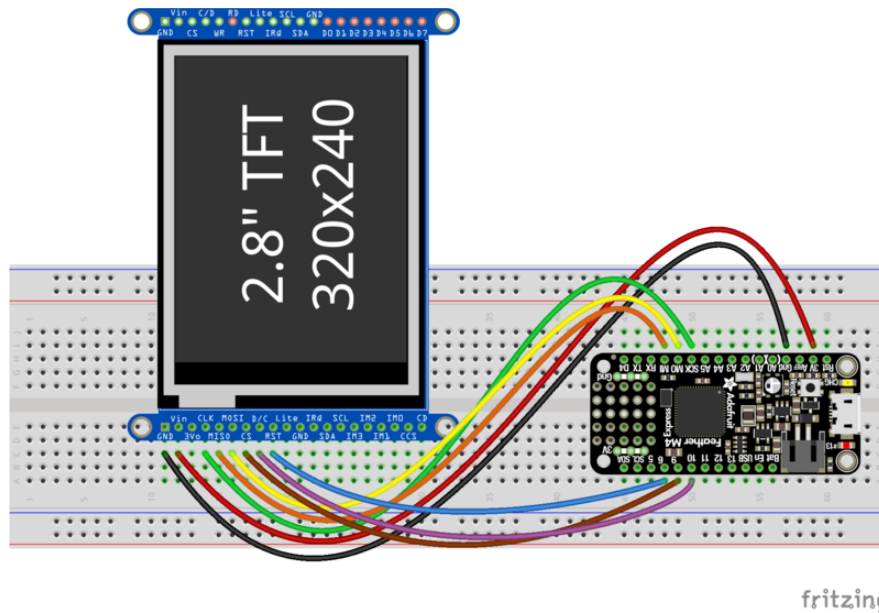
2.8-breakout-feather-m4.fzz
