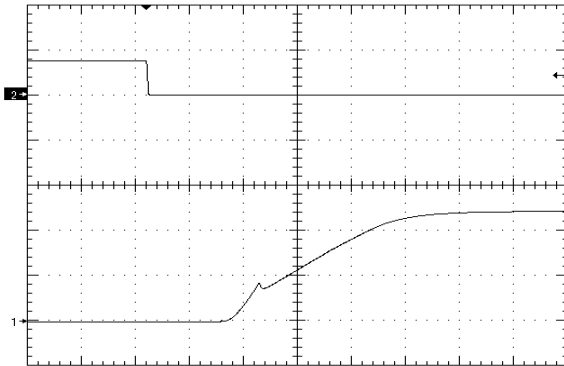
Figure 9. Startup Waveform via Enable Pin, time scale 4mS/div. Vin=Vin_nom, full resistive load (negative enable.) Ch1=2V/div,Ch2=5V/div
