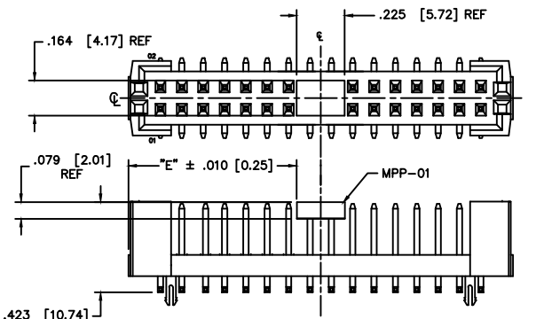
FIG. 5 -M OPTION E = ((\text{No. OF POS.} \times .100 [2.54]) + .200 [5.08]) / 2 - .1125 [2.86]
