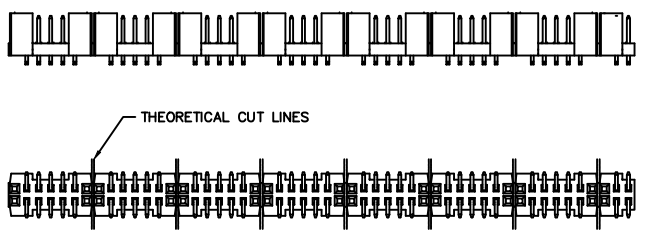
FIG. 3 SCALE: .5X FULL STRIP VIEW
