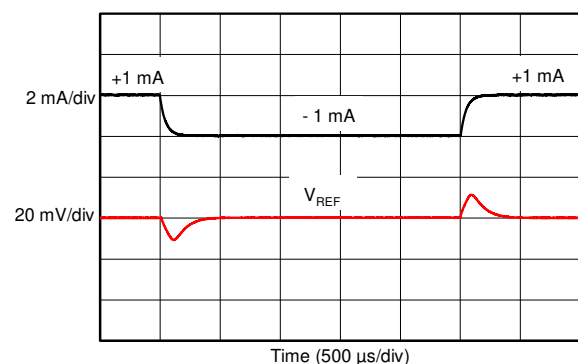
Figure 7-24. Load Transient Response
