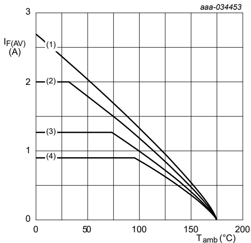
FR4 PCB, mounting pad for cathode 1 cm 2 T_j = 175^\circ\text{C} (1) \delta = 1 ; DC (2) \delta = 0.5 ; f = 20 kHz (3) \delta = 0.2 ; f = 20 kHz (4) \delta = 0.1 ; f = 20 kHz
