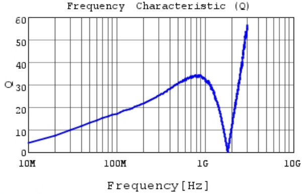
LQG15WZ56NG02 Q
