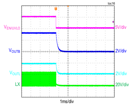
CONDITIONS: PWM MODE, V_{OUTB} = 3.3V , V_{OUTL} = 1.8V , I_{OUTB} = 100mA , I_{OUTL} = 50mA , f_{SW} = 375kHz
