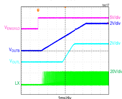
CONDITIONS: PWM MODE, V_{OUTB} = 5V , V_{OUTL} = 3.3V , I_{OUTB} = 100mA , I_{OUTL} = 50mA , f_{SW} = 570kHz
