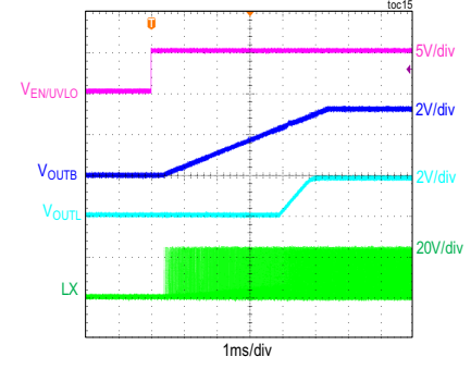
CONDITIONS: PWM MODE, V_{OUTB} = 3.3V , V_{OUTL} = 1.8V , I_{OUTB} = 100mA , I_{OUTL} = 50mA , f_{SW} = 375kHz
