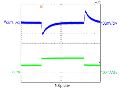
CONDITIONS: PWM MODE, V_{OUTB} = 3.3V , f_{SW} = 375kHz LOAD STEP BETWEEN 75mA TO 150mA
