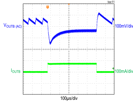
CONDITIONS: PFM MODE, V_{OUTB} = 3.3V , f_{SW} = 375kHz LOAD STEP BETWEEN 5mA TO 75mA
