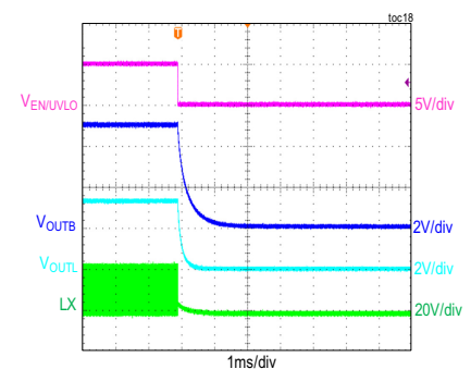
CONDITIONS: PWM MODE, V_{OUTB} = 5V , V_{OUTL} = 3.3V , I_{OUTB} = 100mA , I_{OUTL} = 50mA , f_{SW} = 570kHz
