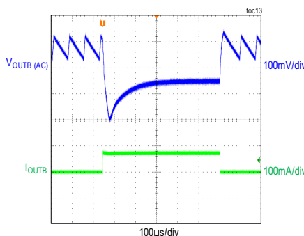
CONDITIONS: PFM MODE, V_{OUTB} = 5V , f_{SW} = 570kHz LOAD STEP BETWEEN 5mA TO 75mA
