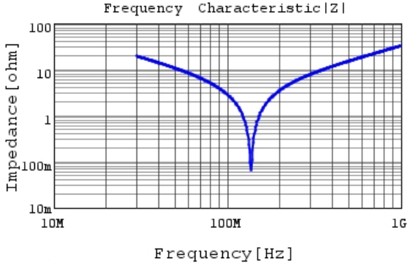
RCE5C2J271J1K1H03B |Z| DC0V, 25degC
