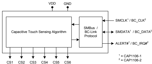
CAP1106 BLOCK DIAGRAM
