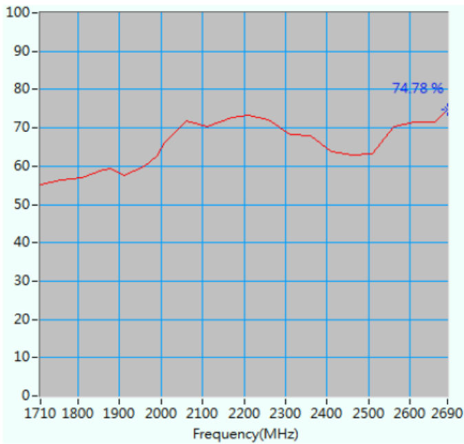
Maximum Efficiency at 2690 MHz : 74.7 %
