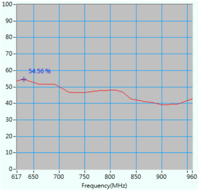
Maximum Efficiency at 630 MHz : 54.5 %
