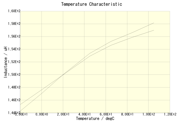
CLF7045T-151M-CA(DC = 0A)
