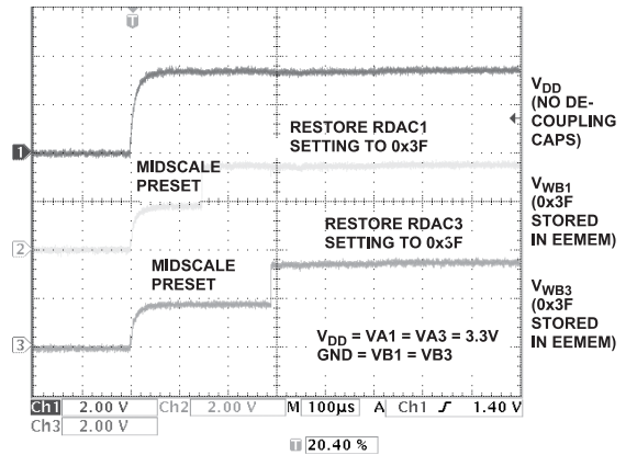
Figure 20. t_{EEMEM\_RESTORE} of RDAC1 and RDAC3
