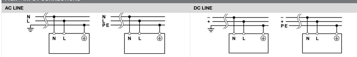
FIG.7 - INPUT CONNECTIONS
