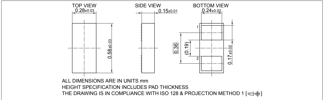
Figure 10 WLL-2-3 package
