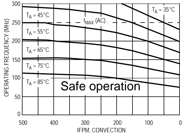
Figure 5. Maximum MPC941 frequency, V_{CC} = 3.3\text{ V} , MTBF 9.1 years, 4 pF load per line
